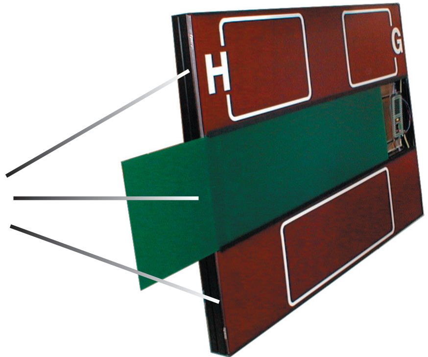
Fig. 1 Sample score-board
